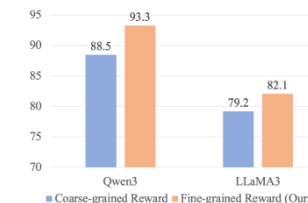
(a) Performance on FDD-ANT.
