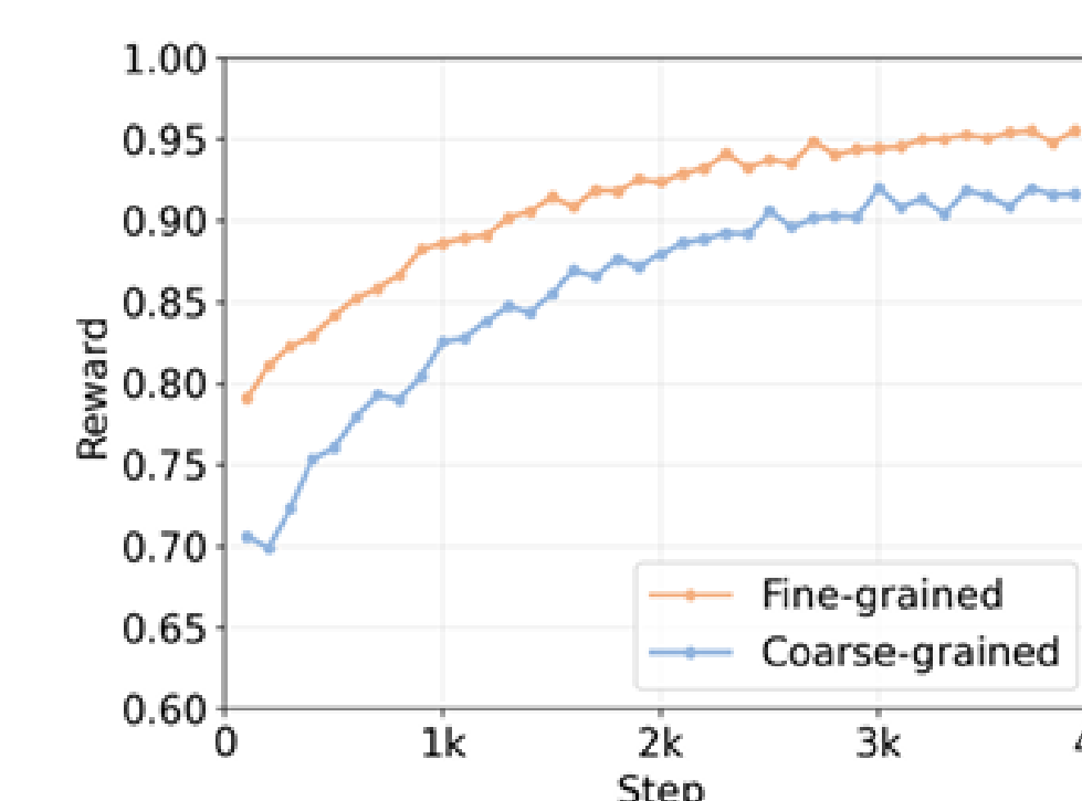
(b) Reward during training.
